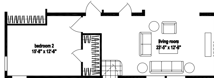
OPTION 2 BEDROOM CONFIGURATION
