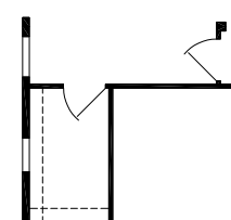
6'-8" 9'-4" OPT SUN ROOM
