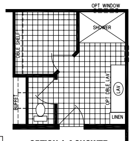
OPTION 4x6 SHOWER (ALSO USE FOR SPRINGVIEW PACKAGE)
